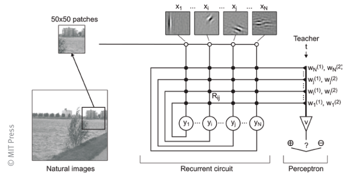
Schematic representation of the model. The image is separated into sub-components, which are then analyzed in a recurrent network. The read-out neuron (at the right) classifies the image into two categories (+ or -)
