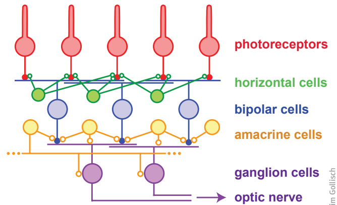
Schematic representation of the structure of the retina
